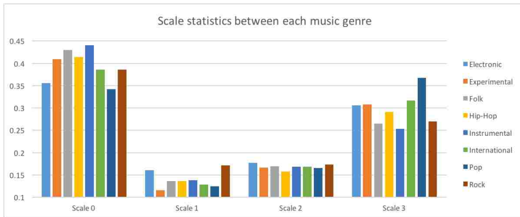
Figure 5.3: Statistics of scale selections between each music genre. The height of each bar indicates the ratio of how much times the scale is selected in the corresponding genre. Best viewed in colors.
